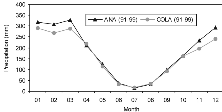
Fig. 5 Monthly mean precipitation variation of long period at the study area (1991–1999).
