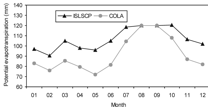
Fig. 6 Monthly mean potential evapotranspiration variation at the study area (1986–1990).
