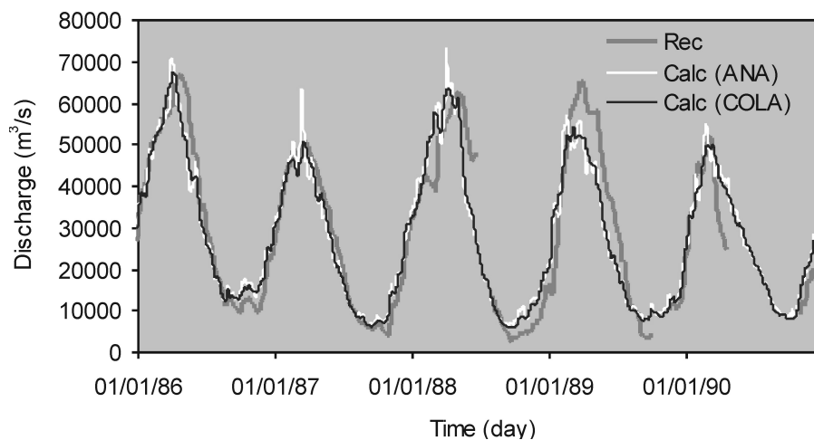
Fig. 7 Recorded and calculated discharge at Fazenda Vista Alegre.
