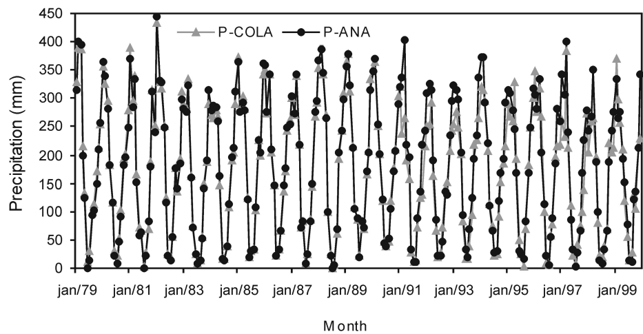
Fig. 3 Monthly mean precipitation at the study area for the period 1979–1999.
