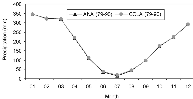
Fig. 4 Monthly mean precipitation variation of long period at the study area (1979–1990).
